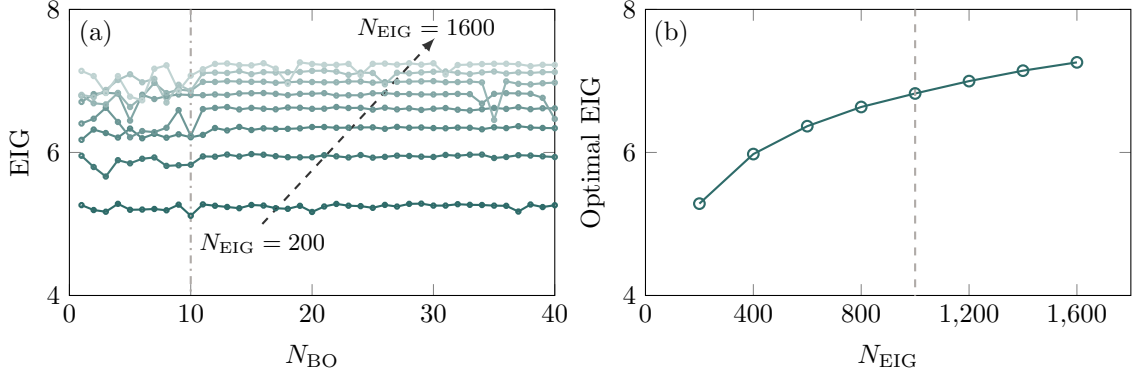
Figure 2: BO output trajectories (a) and the optimal BO outputs (b) for EIG sample sizes N_{\text{EIG}} = 200, 400, \dots, 1600 . The dot-dashed line in (a) indicates the onset of the BO process with 10 initial trials. The optimal EIG for the EIG sample size used later, N_{\text{EIG}} = 1000 , is highlighted in (b).
