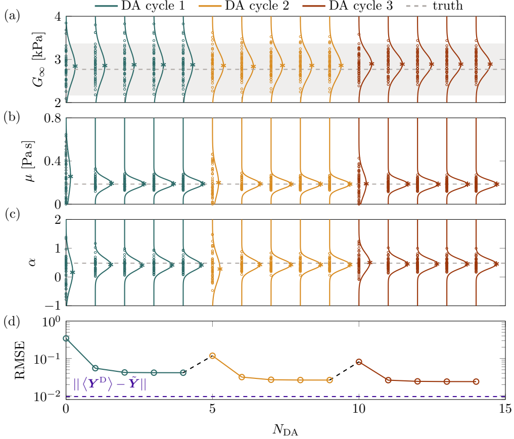
Figure 3: DA outputs over the total En4D-var iteration number N_{DA} : ensembles for (a) G_\infty ; (b) \mu ; (c) \alpha ; and (d) RMSE of the bubble dynamics curves. The shaded area in (a) represents the 95% confidence interval for the G_\infty measurements. The solid curves in (a–c) represent Gaussian distributions approximated from the 48 ensembles, with their respective mean values marked as stars. In (d), the error between the mean of the measurements and the unobtainable truth, \|\langle \mathbf{Y}^D \rangle - \tilde{\mathbf{Y}}\| , is shown for comparison.
