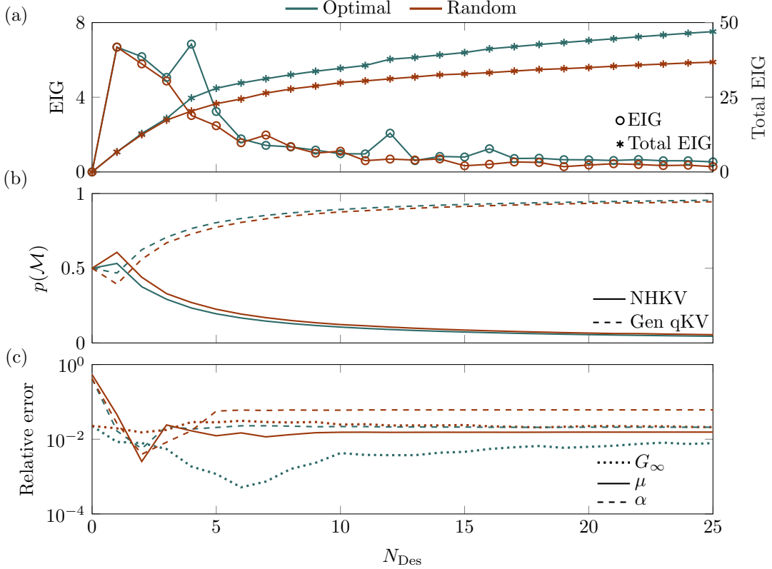
Figure 5: Sequential BOED outputs over the design number N_{\text{Des}} : (a) EIG and total EIG; (b) model probabilities; and (c) relative error of the mean material properties.
