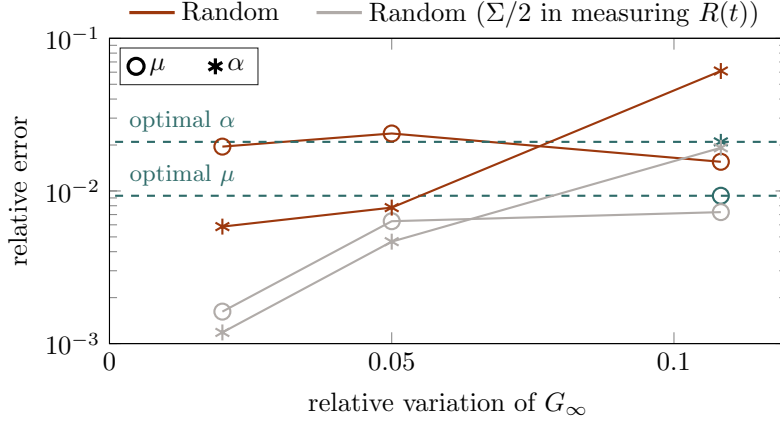
Figure 6: Convergence study of different error sources.
