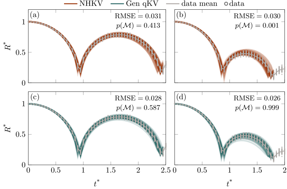
Figure 4: Posterior bubble dynamics trajectories and their marginal likelihoods: (a, c) R_{\max} = 9.85 \times 10^{-4} m and R_{\infty}^* = 0.2887 ; (b, d) R_{\max} = 3.87 \times 10^{-4} m and R_{\infty}^* = 0.15 .
