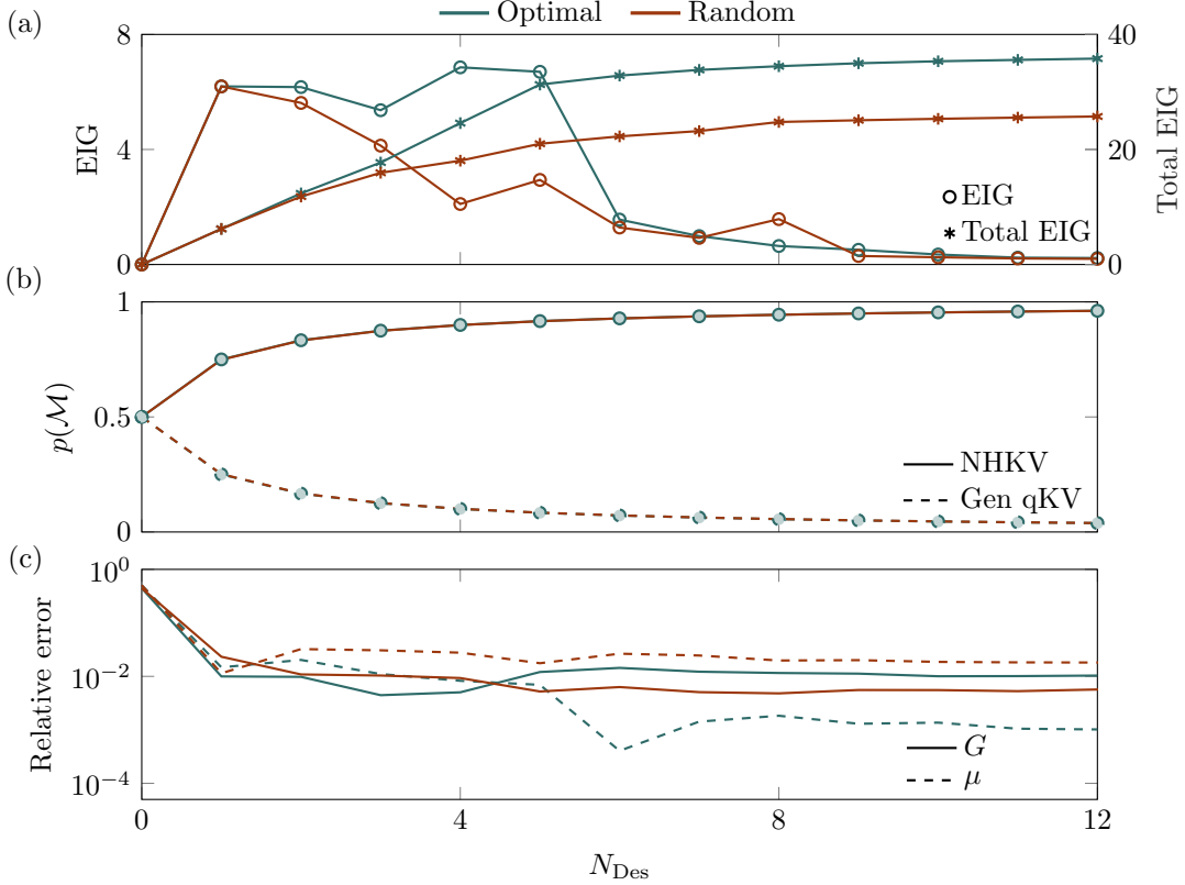
Figure 7: Sequential BOED outputs over the design number N_{\text{Des}} : (a) EIG and total EIG; (b) model probabilities p(\mathcal{M}) ; and (c) relative error of the mean material properties.
