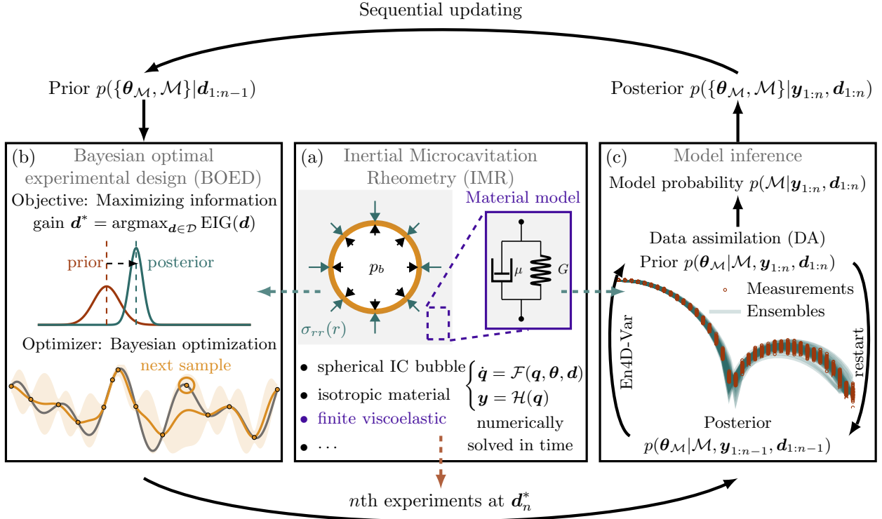
Figure 1: Schematic of the IMR-based sequential BOED. Given a modeling parameter, \theta = \{\mathcal{M}, \theta_{\mathcal{M}}\} , which includes a constitutive model and its material properties, and a design \mathbf{d} that describes the experimental setup (e.g., the equilibrium radius), the IMR approach numerically solved the spherically symmetric motion of bubble dynamics. In computation, the complete flow states \mathbf{q} include bubble radius, bubble-wall velocity, temperature, and other variables, but they are only partially observable and are denoted as \mathbf{y} .
