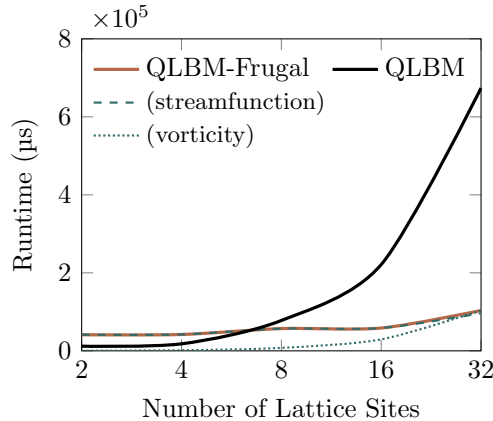
Figure 14: Runtime estimation for the proposed D2Q5 QLBM-frugal algorithm without quantum bounds, compared against the QLBM algorithm proposed by Budinski [50]. The circuit is transpiled with optimization level 3 on the IBM Brisbane backend.
