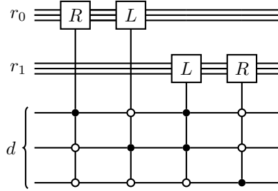
Figure 5: Streaming for a two-dimensional lattice grid. The streaming step uses right and left shift operators R and L to shift distributions in their respective link directions \alpha_1 and \alpha_2 by controlling the gates on qubits in each link register d .
