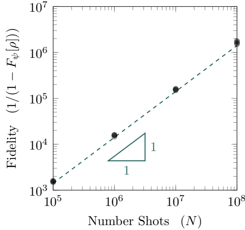
Figure 10: Verification via linear convergence with shot number of the advection–diffusion D1Q3 algorithm.
