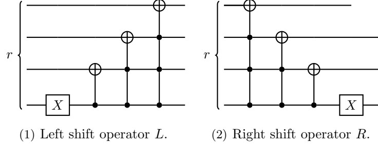
Figure 4: Circuit decomposition for (a) left shift and (b) right shift operators. These gates are applied to qubits in r_1 for left and right shifts and qubits in r_2 for up- and down-shifts.
