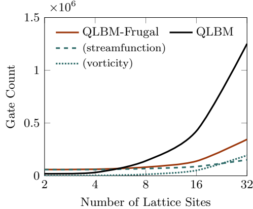
Figure 13: Comparison of costly two-qubit gate counts on the D2Q5 algorithm for the proposed two-circuit approach against Budinski [50]’s algorithm. Transpiled on the IBM Brisbane backend. The horizontal axis “Number of Lattice Sites” scales logarithmically.
