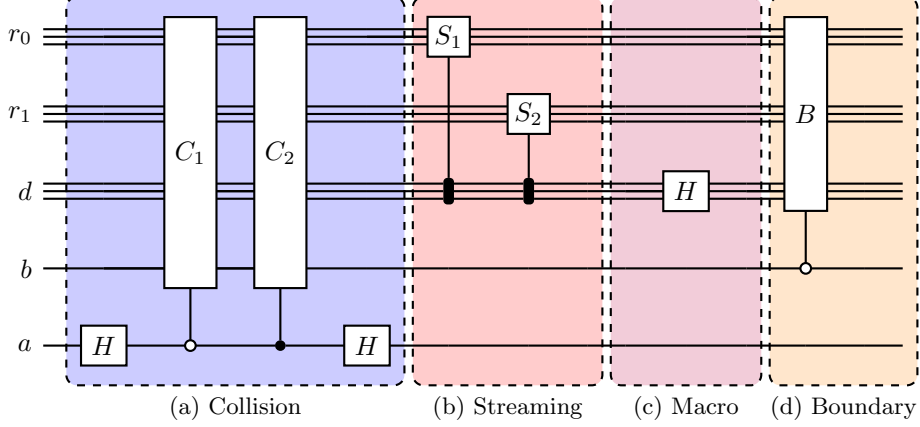
Figure 6: The original D2Q5 vorticity circuit proposed by Budinski [50], modified from the generalized circuit in fig. 2 for boundary conditions. The changed circuit includes an additional qubit b to store the boundary conditions and computations. We propose an algorithm that splits this circuit into two distinct parts.
