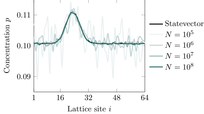
Figure 9: The results of the D1Q3 algorithm at iteration 50 are obtained via finite sampling of the quantum circuit at various sample sizes N_{\text{samp.}} .
