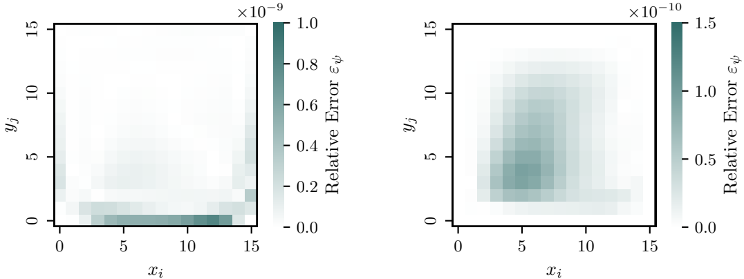
(a) Relative error \varepsilon_\omega for vorticity circuit (b) Relative error \varepsilon_\psi for stream function circuit
