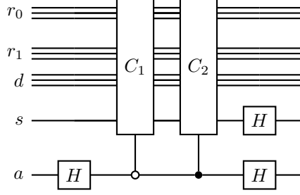
Figure 7: Collision portion of the stream function circuit. An additional qubit s stores the source term, and an additional Hadamard gate on qubit s after the block encoding adds the source term to the link distributions \alpha_i before streaming.
