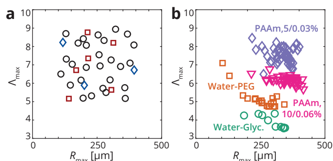
Fig. 7 Distribution of \{R_{\max}, \Lambda_{\max}\} in (a) synthetic experiments and (b) LIC experiments. For synthetic experiments, all data points are considered in the n = 36 case, the red square and bubble diamond points are considered in the n = 9 case, and only the blue diamond points are considered in the n = 3 case.
